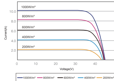
I-V CURVES OF PV MODULE(345W)
